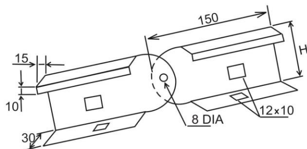
ADJUSTABLE VERTICAL JOINT
